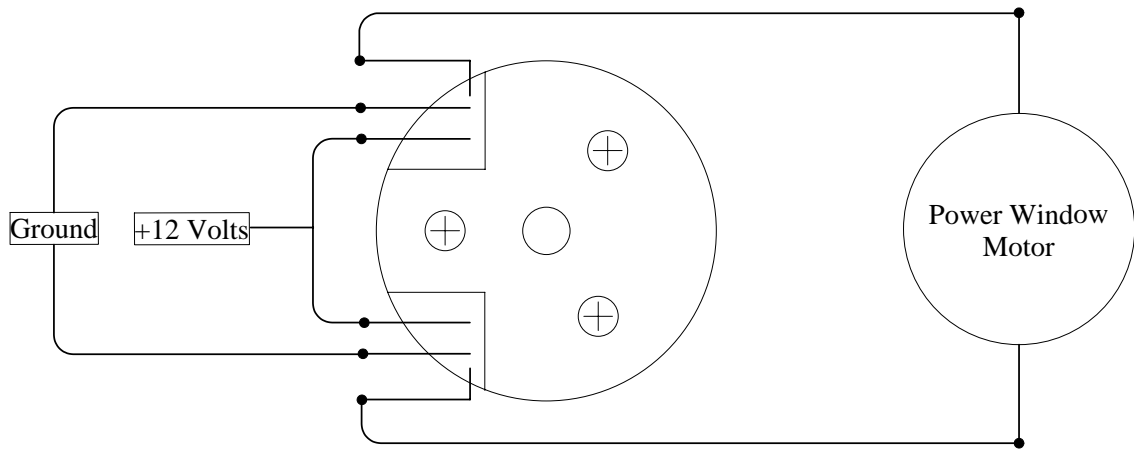
Connection for Two Wire Motor
